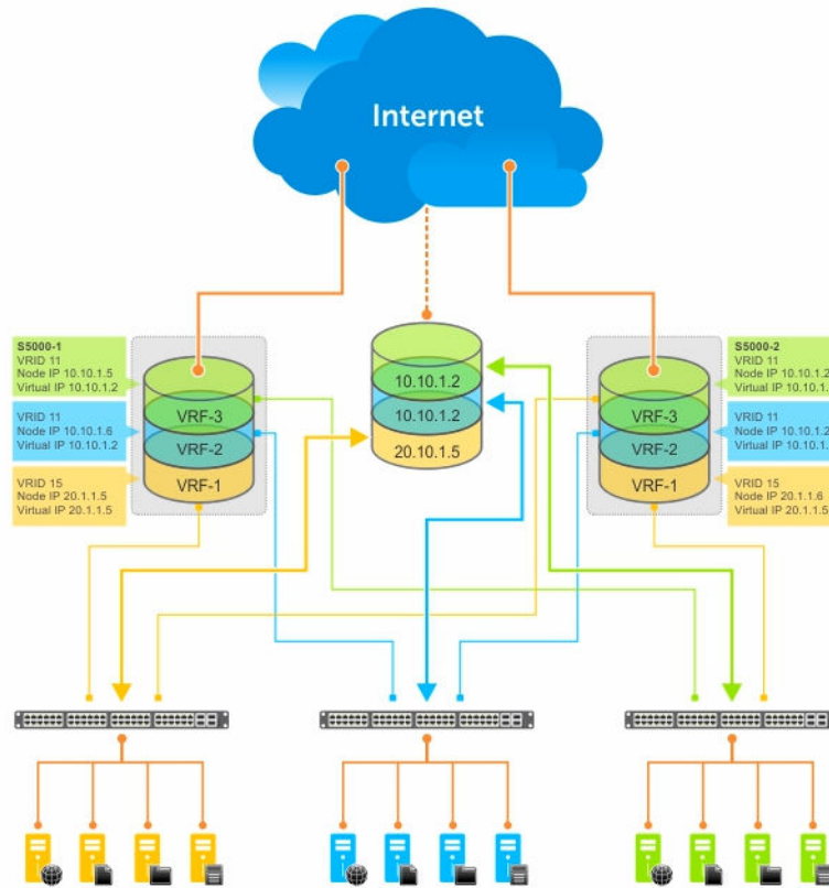
Figure 128. VRRP in a VRF: Non-VLAN Example
